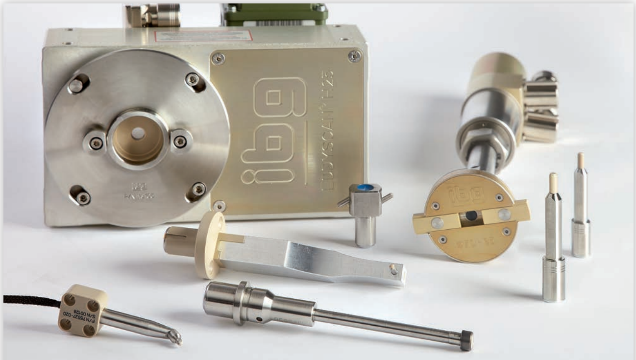
Highest test reliability and sensitivity - different kinds of probes for crack and grinder burn detection. Back left a rotating head eddyscan H for testing a string of parts and bars, back right a rotating head eddyscan F for testing of boreholes and surfaces.
