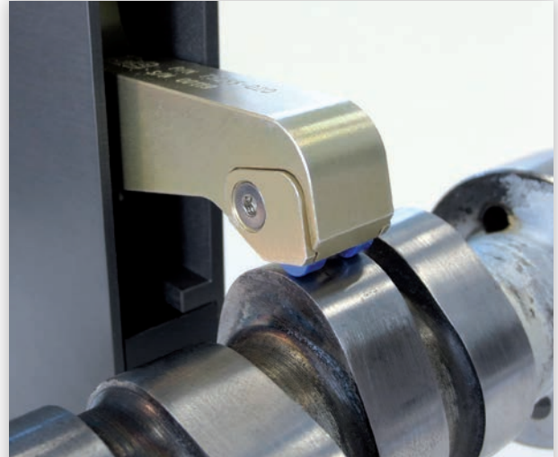
Crack detection probe box for contacting testing on eccentric parts like camshaft lobes for cracks and grinder burn; large diameter range is covered; up to 300 rpm (depending of part geometry), ceramic supports for long life-time. Solutions for structure test on camshafts on request.
